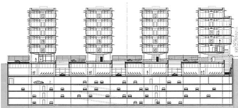
Figure 4: Elevation view of the new buildings
