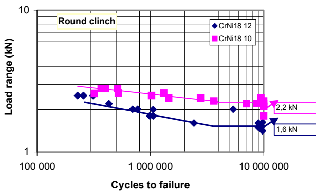
Figure 23 S-N curves for 1 mm clinched lap shear joints. From Ref.(13).
