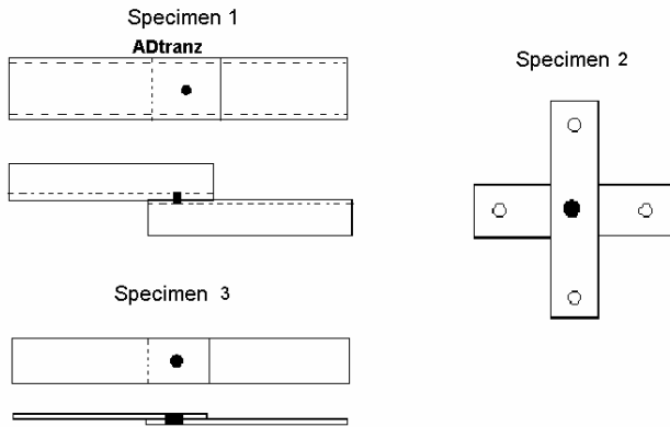
Figure 3 Lap joint specimens used to study spot welding, adhesive bonding and weldbonding.
