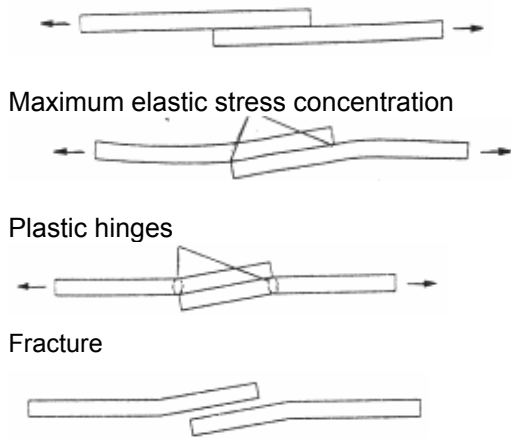
Figure 1 Deformation of lap joint during loading.
