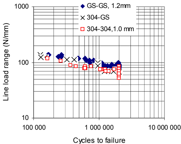
Figure 19 Fatigue of dissimilar metals spot welds. AISI 304 to galvanised mild steel.
