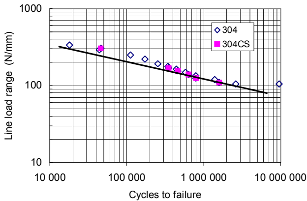
Figure 14 Fatigue properties for 4 mm AISI 304 at two strength levels. The joints consist of two rows of spot welds 60 mm apart.
