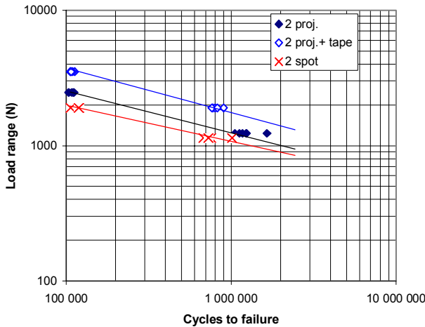
Figure 11 Fatigue properties for spot welded and projection welded, with and without adhesive tape, 0.8 mm temper rolled AISI 301. The loads refer to a specimen with two nuggets.
