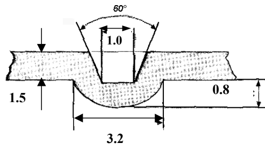
Figure 9 The projection and its dimension in mm.
