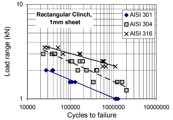
Figure 22 Fatigue properties of rectangular clinched stainless steel sheets.
