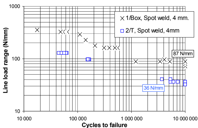
Figure 15 Fatigue results for 4 mm, spot welded SAF 2304 duplex stainless steel. 2/T indicates transverse loaded specimen type 2. All at 10^7 were runouts.
