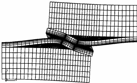
Figure 2 FEM analysis of spot-welded joint showing rotation of joint (1).
