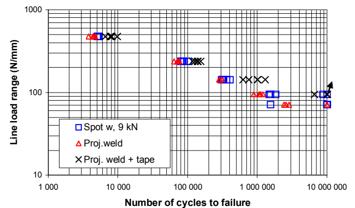
Figure 10 Fatigue results from spot and projection welded single spot welded joints of temper rolled AISI 301. 6.8 mm nugget diameter.
