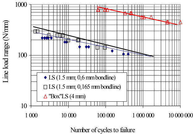
Figure 25 S-N curve for 4 mm flanged specimen type 1 and 1.5 mm specimen type 3 with bondline thickness of 0.165 and 0.6 mm. Bonded with toughened epoxy system, DP 490. (Room temperature, 20 Hz, R = 0.1)
