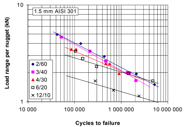
Figure 12 Fatigue results for multiple spot welded joints of 1.5 mm AISI 301 at 417 MPa yield strength level. Code: No of nuggets /Pitch. Recalculated from Ref.(7).
