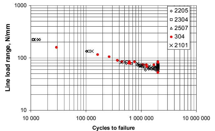
Figure 16 Line load range versus cycles to failure graph for resistance spot welded 1mm thick duplex stainless steels compared to 1mm, AISI 304, all in annealed condition. All at 2 \times 10^6 were runouts.
