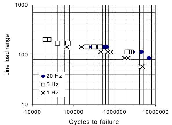
Figure 28 Fatigue of 1.5 mm AISI 304L stainless steel adhesive joints. Effect of loading frequency.
