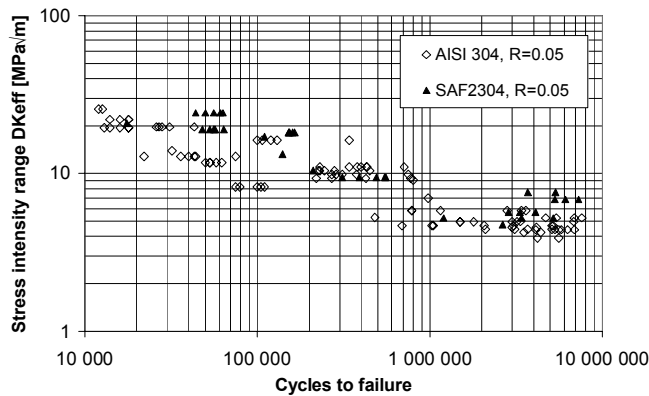
Figure 7 Stress intensity ranges versus number of cycles to failure for specimen types 1 and 2, all sheet thickness and with steel grades separated.
