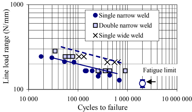
Figure 31 S-N curves for 3 mm AISI 304 laser welded simple lap shear joints. Controlled penetration.
