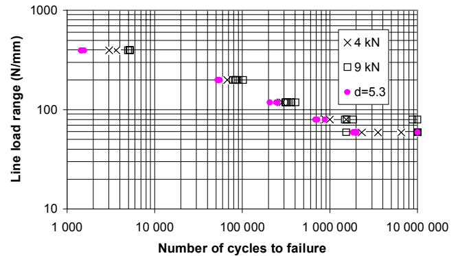
Figure 8 Fatigue properties of spot-welded temper rolled AISI 301. The two series with different clamping forces both had 6.4 mm diameter nuggets.
