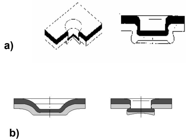
Figure 20 Perspective view and cross section of a) Round clinch element and b) Rectangular, partly sheared clinch (12).
