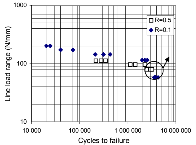
Figure 27 Fatigue of 1.5 mm AISI 304L stainless steel adhesive joints. Effect of load ratio.
