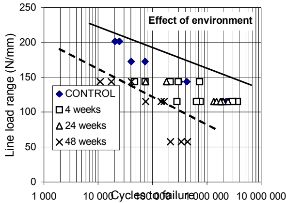
Figure 29 Fatigue of 1.5 mm AISI 304L stainless steel adhesive joints. Specimen immersed in water for 4 to 48 weeks.
