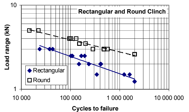
Figure 24 Fatigue properties of rectangular and round clinched stainless steel sheets. 1 mm AISI 304
