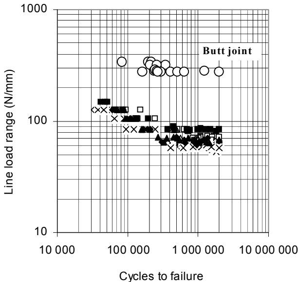
Figure 32 Fatigue properties of laser welded lap joints.
