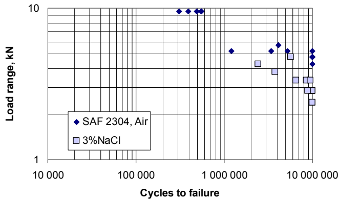
Figure 18 Effect of 3% NaCl environment on fatigue properties of spot welded duplex SAF 2304 stainless steel. 10^7 cycles life are all run-outs.
