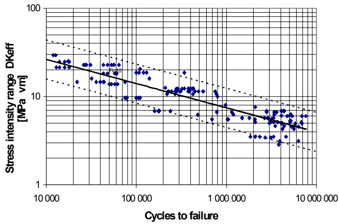
Figure 6 Stress intensity ranges versus number of cycles to failure for all specimen types, sheet thickness and steel grades. 95% confidence limits are shown.
