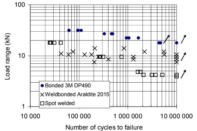
Figure 30 S-N curve for 4 mm flanged simple lap joint weldbonded with toughened epoxy system Araldite 2015. (Room temperature, 50 Hz, R = 0.05). Comparative data from Ref. (3) and (15).
