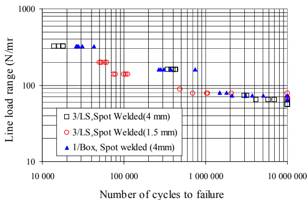
Figure 4 Fatigue properties of spot welded AISI 304CS.
