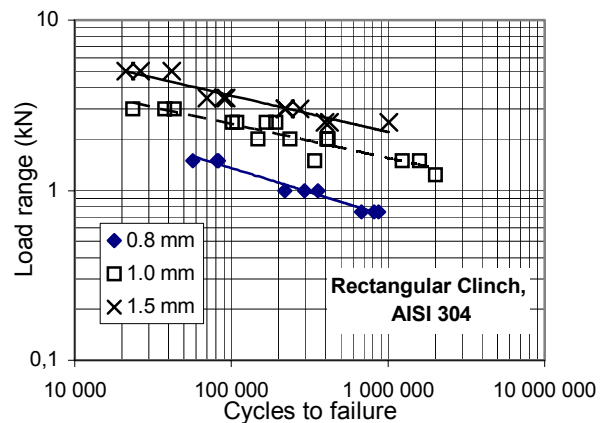
Figure 25 Fatigue properties of rectangular clinched stainless steel sheets in three different thicknesses.
