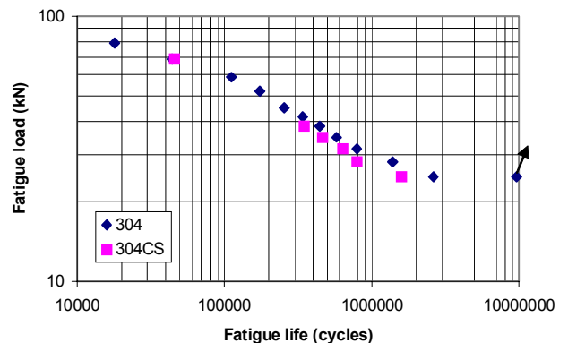
Figure 13 Fatigue results for multi-spot 4 mm AISI 304 in annealed and cold stretch condition (304CS). Each specimen has 4 nuggets.
