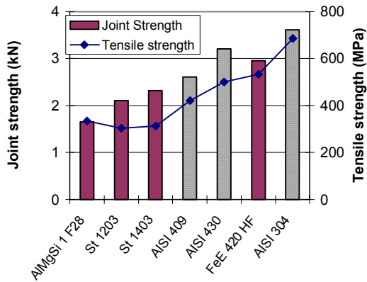
Figure 21 Clinch joint strength and tensile strength for different 1 mm sheet materials (12).
