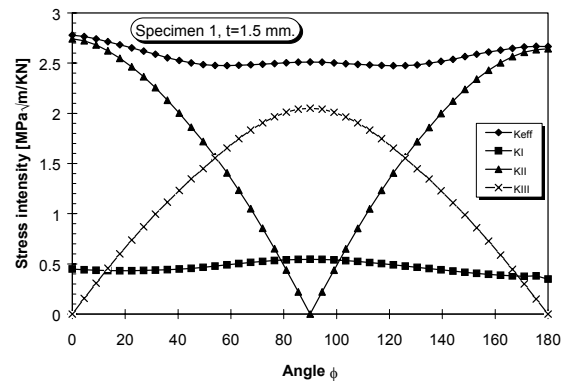
Figure 5 Variation of stress intensity factor for type 1 specimen.
