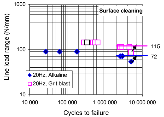
Figure 26 Fatigue of 1.5 mm AISI 304L stainless steel adhesive joints. Effect of surface cleaning.
