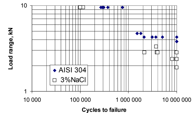
Figure 17 Effect of 3% NaCl environment on fatigue properties of spot welded AISI 304 stainless steel. 10^7 cycles life are all run-outs.
